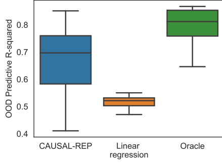
(a) Supervised CAUSAL-REP: Toy synthetic data
