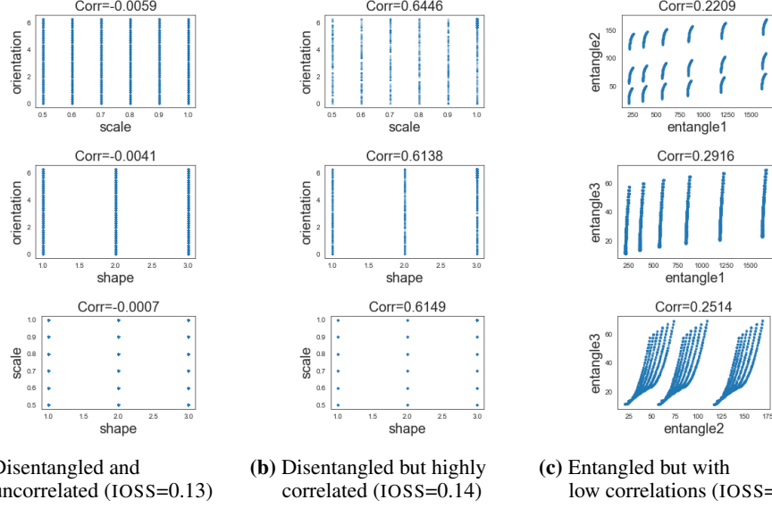
Figure 8: Disentangled features have independent support even though they may be correlated. Moreover, the independence of support can distinguish disentangled and entangled features. This figure illustrates how entangled and disentangled features differ using pairwise scatter plots. Figure 8a considers the ground truth features (shape, scale, orientation) of the dSprites dataset. These features are disentangled. They also have independent support; e.g., conditional on ‘scale’, the set of values that ‘orientation’ can take does not change with ‘scale.’ Visually, these disentangled features have scatter plots that occupy rectangular (or hyperrectangular) regions. Figure 8b considers the same features but in a subset of the dSprites dataset where the features are correlated. These features, though correlated, are still disentangled; they also have independent support. Figure 8c considers three entangled features, each of which is a nonlinear transformation of the three ground-truth features. These features are not disentangled. Their supports are also not independent. Conditional on ‘entangle1’, the possible values ‘entangle2’ can take depends on the value of ‘entangle1.’
