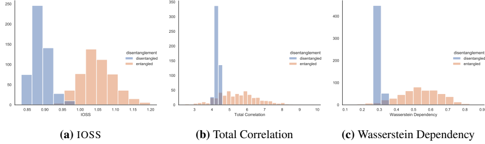
Figure 9: IOSS can better distinguish entangled and disentangled representations than existing unsupervised disentanglement metrics on the mpi3d dataset.
