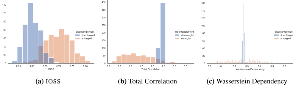
Figure 15: IOSS can better distinguish entangled and disentangled representations than existing unsupervised disentanglement metrics on the smallnorb dataset.
