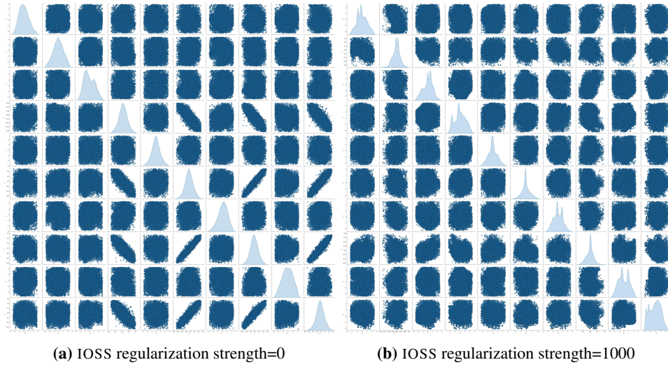
Figure 17: Increasing regularization strengths of IOSS encourages the learned representation to have independent (i.e. hyperrectangular) support. (a) The pairwise scatter plot of the learned representations without IOSS regularization; some dimensions of the representation do not have independent support. (b) The pairwise scatter plot of the learned representations with IOSS regularization; most dimensions of the representation have independent support.
