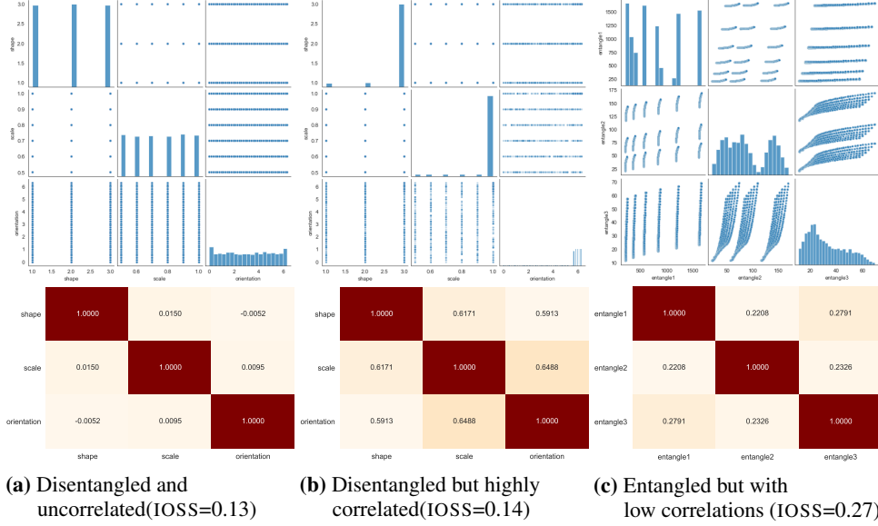
Figure 13: Disentangled features have independent support even though they may be correlated. Moreover, IOSS can distinguish disentangled and entangled features. This figure illustrates how entangled and disentangled features differ using pairwise scatter plots. Figure 13a considers the ground truth features (shape, scale, orientation) of the dsprites dataset. These features are disentangled. They also have independent support, e.g., conditional on ‘scale’, the set of values that ‘orientation’ can take does not change with ‘scale.’ Visually, these causally disentangled features have scatter plots that occupy rectangular (or hyperrectangular) region. Figure 13b considers the same features but in a subset of the dsprites dataset where the features are correlated. These features, though correlated, are still disentangled; they also have independent support. Figure 13c considers three entangled features, each of which is a nonlinear transformation of the three ground-truth features. These features are not disentangled. Their support are also not independent. Conditional on ‘entangle1’, the possible values ‘entangle2’ can take depends on the value of ‘entangle1.’
