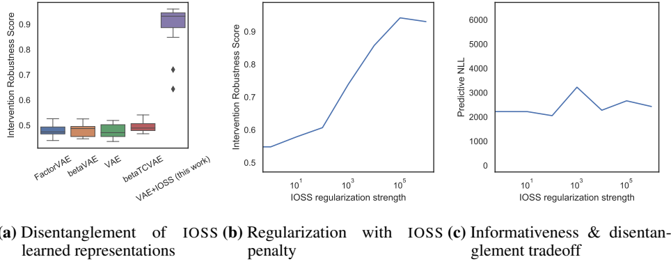
Figure 10: (a) VAE+IOSS outperforms existing unsupervised disentanglement algorithms in producing representations that are more causally disentangled. (b) Regularizing for IOSS encourages learning disentangled representations. The intervention robustness score of the representation increases as we increase the regularization strengths of IOSS. (c) There is no obvious tradeoff between informativeness and disentanglement. The model fit stays stable despite we increase the regularization strengths of IOSS.
