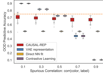
(b) Unsupervised CAUSAL-REP: Colored and Shifted MNIST
