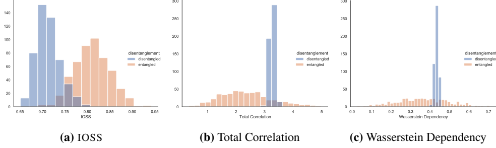
Figure 14: IOSS can better distinguish entangled and disentangled representations than existing unsupervised disentanglement metrics on the dsprites dataset.
