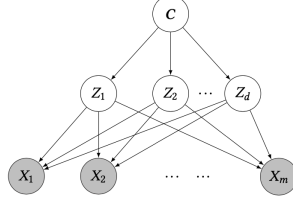
Figure 3: The SCM of unsupervised disentanglement [13].
