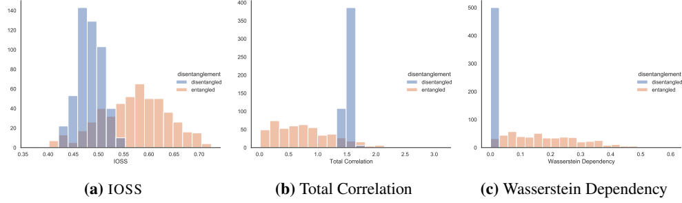
Figure 16: IOSS is competitive in distinguishing entangled and disentangled representations compared with existing unsupervised disentanglement metrics on the cars3d dataset.
