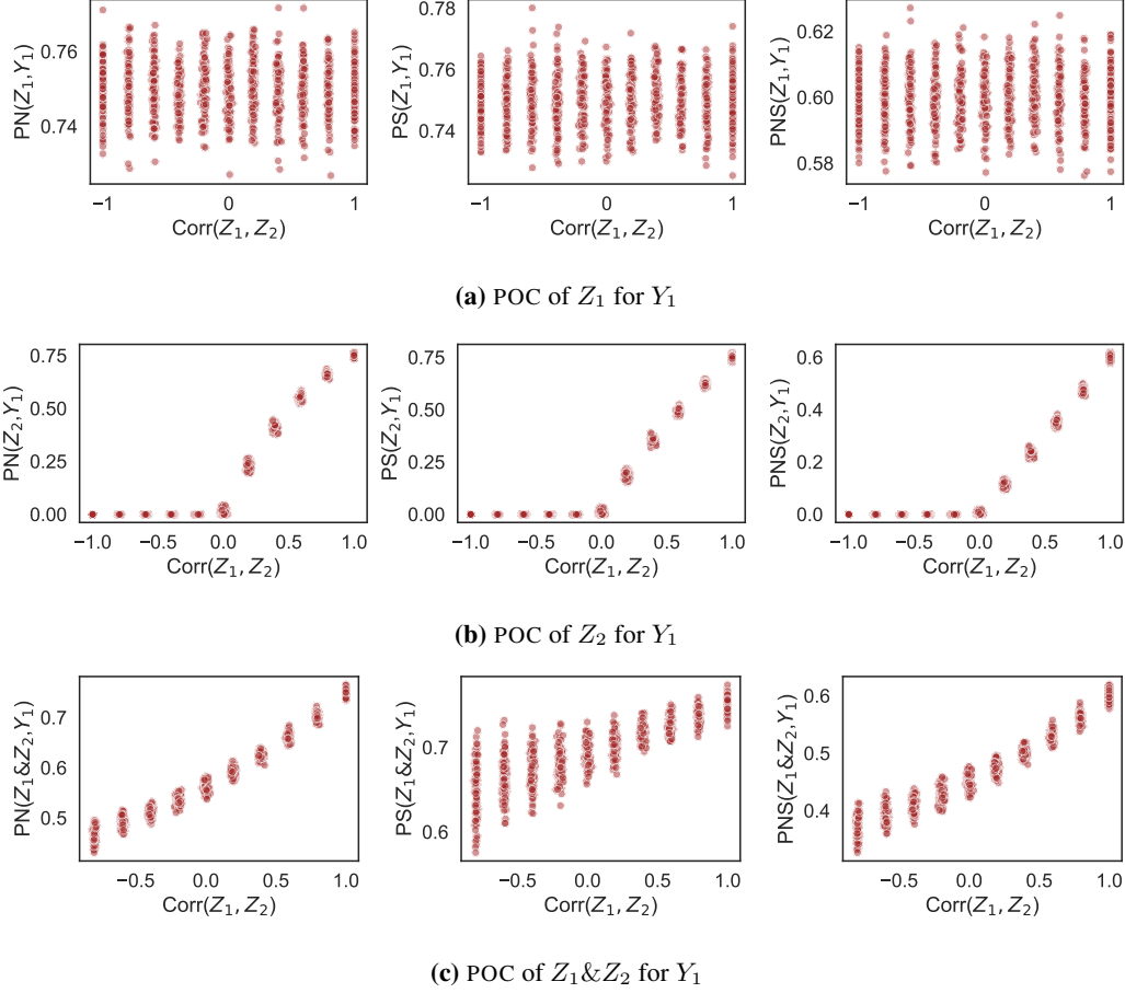
Figure 11: Lower bounds of probabilities of causation are consistent with intuitive notions of feature necessity and sufficiency. As Z_1 and Z_2 become increasingly highly correlated, (a) the POC of Z_1 for Y_1 stays high, (b) the POC of Z_2 for Y_1 starts to increase when the correlation turns positive, and (c) the POC of Z_1 \& Z_2 increases.
